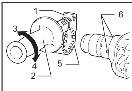
► 1. Grip base 2. Side grip 3. Loosen 4. Tighten 5. Teeth 6. Protrusion
