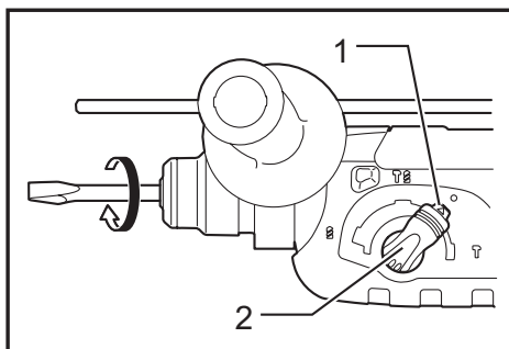
► 1. Lock button 2. Action mode changing knob
